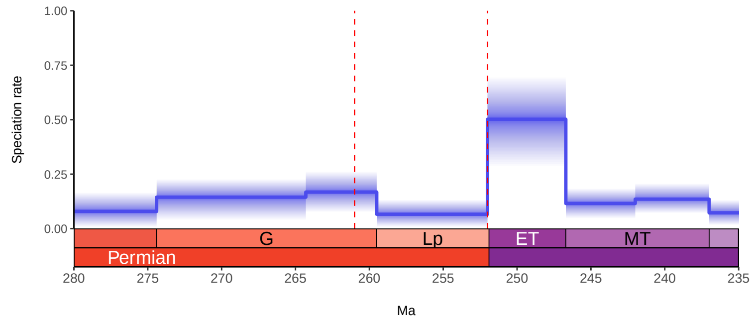
All Reptilia Model 7: BDNN MCMC by Stages with Isotopic Predictors
