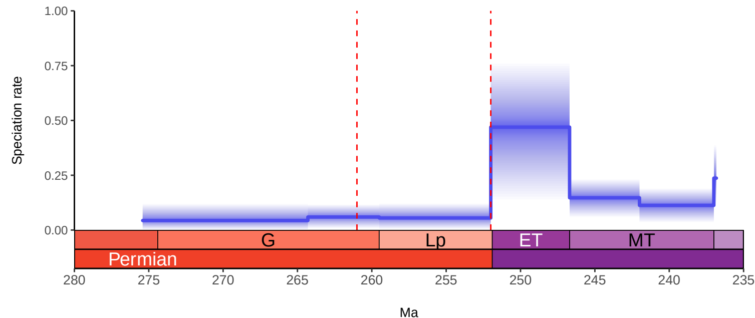
All Reptilia Model 6: BDNN MCMC by Stages with Isotopic Predictors
