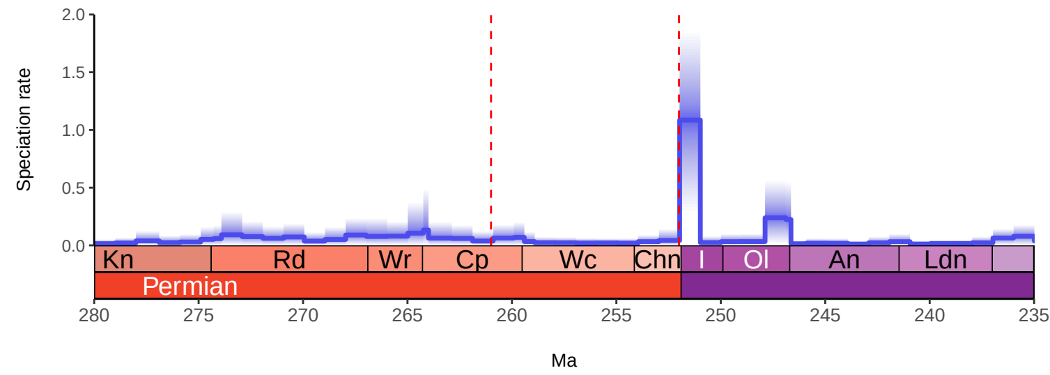
All Reptilia Model 8 NEW PyRate: BDNN MCMC 1Myr w/ Isotopic & Stage Predictors
