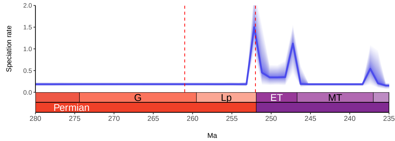
All Reptilia Model 5: RJMCMC by 1Myr with No Predictors
