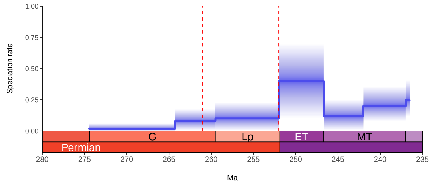
Terrestrial Reptilia Model 4: MCMC by Stages with BRIDGE Predictors
