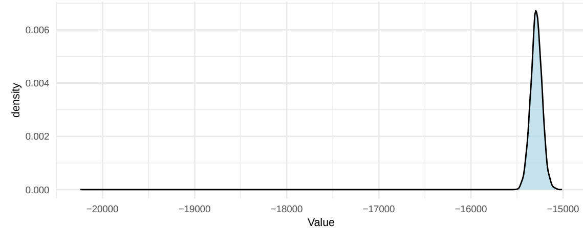
Prior Density
