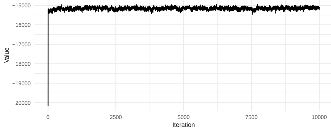
Prior Trace
