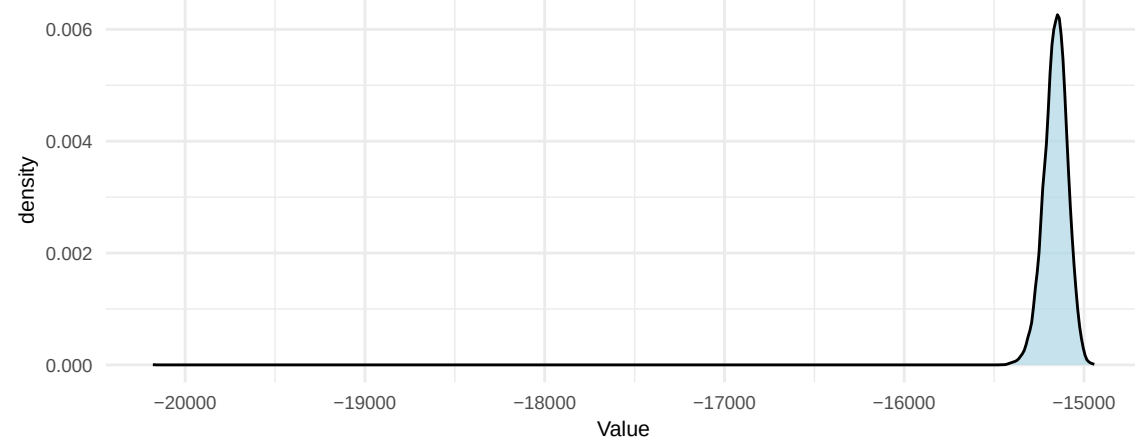
Prior Density
