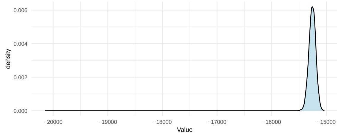
Prior Density
