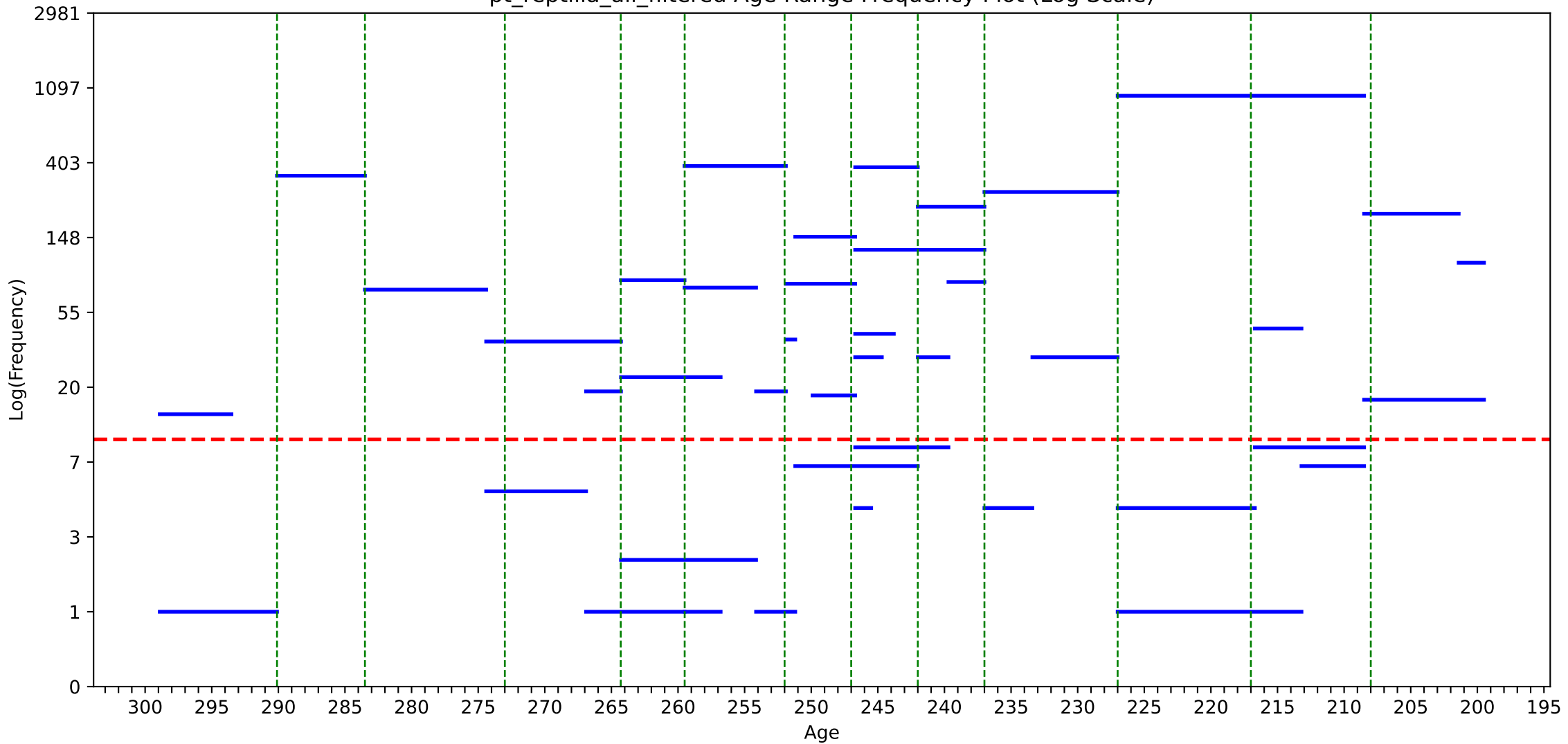
pt_reptilia_all_filtered Age Range Frequency Plot (Log Scale)
