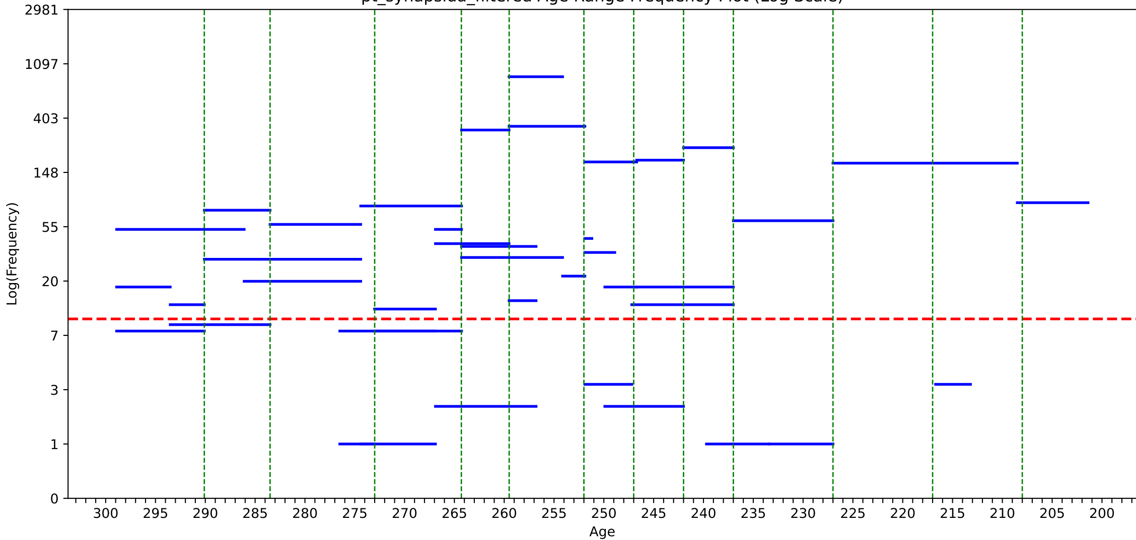
pt_synapsida_filtered Age Range Frequency Plot (Log Scale)
