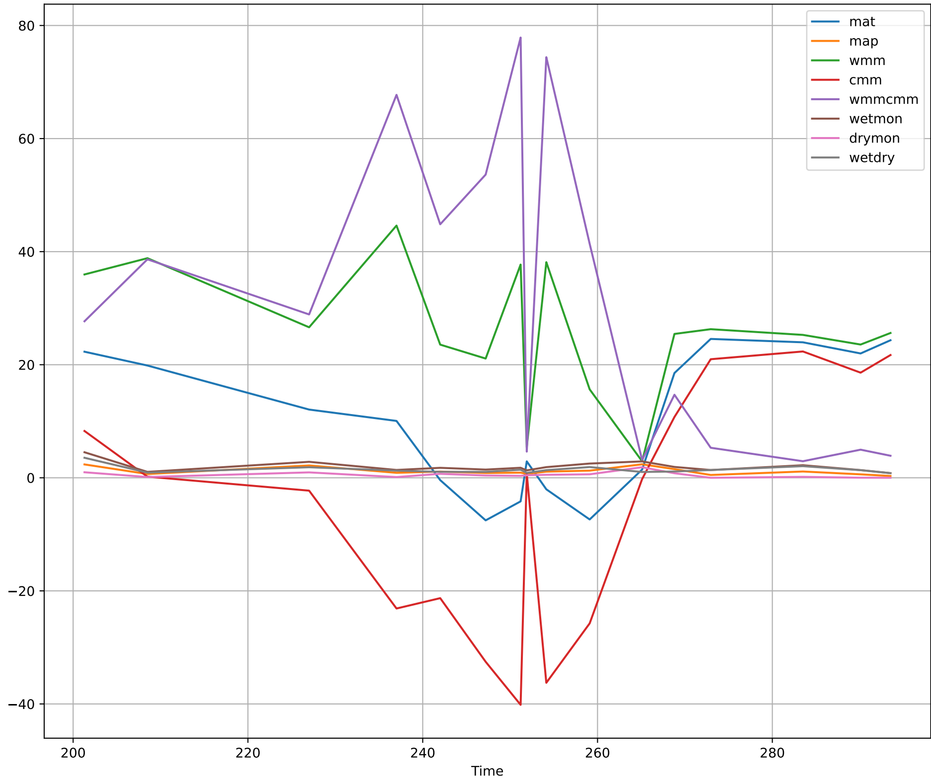
Synapsida Raw Climatic BRIDGE Variables Over Time
