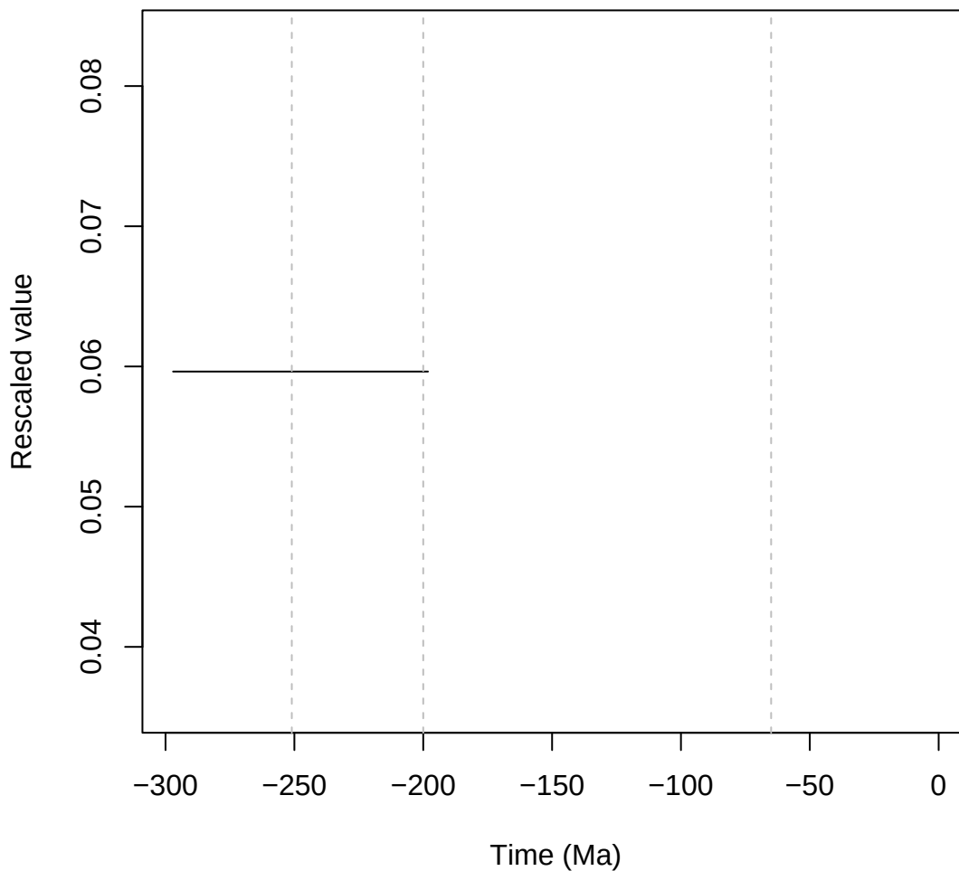
Trajectory of variable: Mod_scaled
