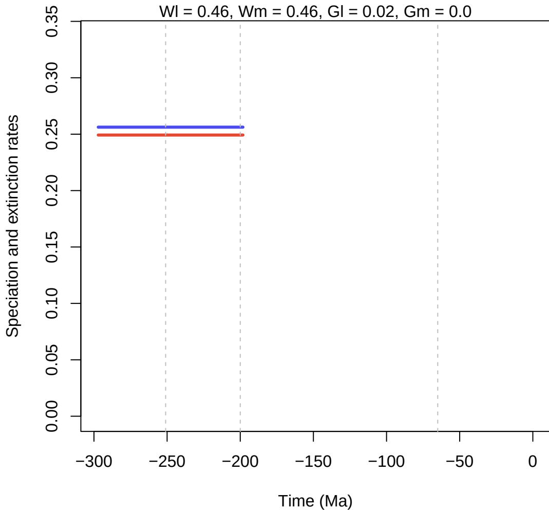
Effect of: Mod_scaled
