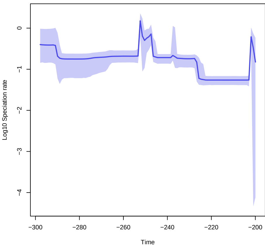
Speciation (combined_7_mcmc)
