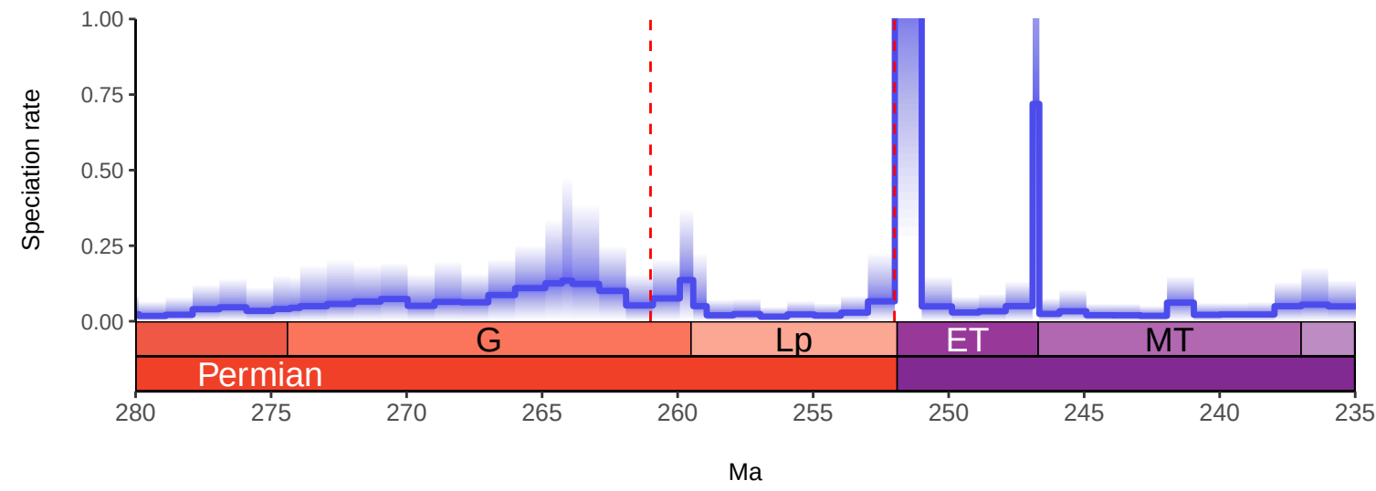
All Reptilia Model 8: BDNN MCMC by 1Myr with Isotopic Predictors
