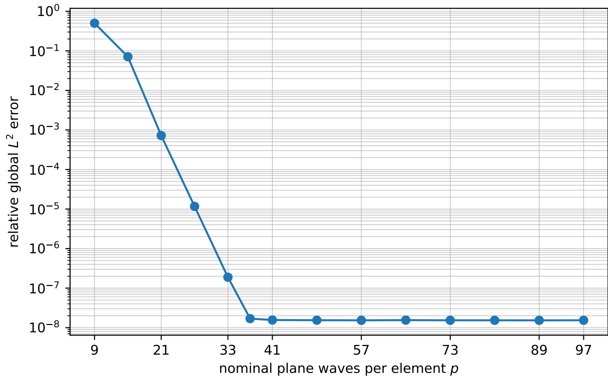
Centered Hankel DtN PWDG at k = 16
