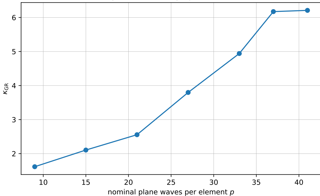
Conditioning of the actual graph-Riesz PWDG solve
