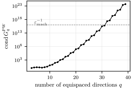
(b) plane-wave trace Gram
