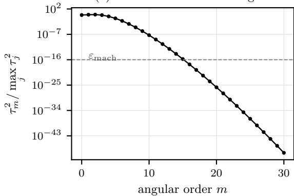
(a) Fourier–Bessel trace weights
