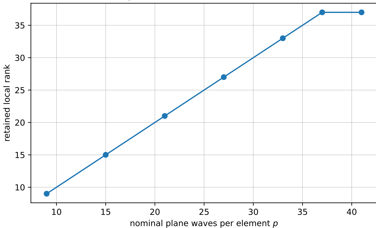
Binary64 trace-rank saturation, \tau = 10^{-12}
