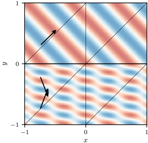
(a) \Re u, \theta_i = 69^\circ (propagating)
