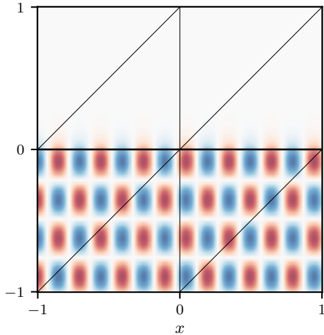
(b) \Re u, \theta_i = 29^\circ (total reflection)
