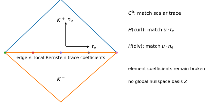
Fig. 1 Smoothness functionals on a pair of triangles. The B-coefficients remain broken. Continuity of a scalar spline matches the coefficients at the shared domain points; tangential continuity of a spline vector field matches the coefficients of the tangential component on the edge; normal continuity matches those of the normal component. No coefficient is identified across triangles.
