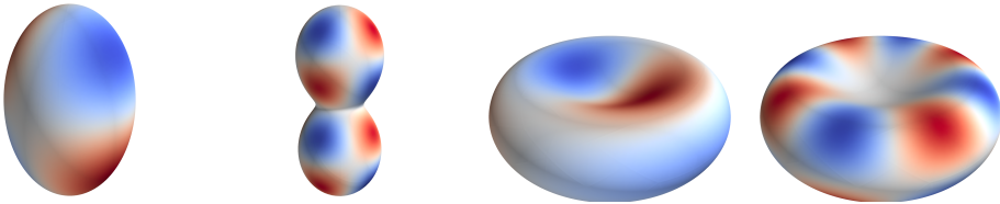
FIG. 1. Computed eigenfunctions at d = 6 , r = 1 , level 2, drawn on the embedded surfaces. From left: spheroid, seventh eigenfunction, \mu = 5.38 ; dumbbell, \mu = 57.62 , with azimuthal and axial nodal lines crossing both bulbs; red blood cell, a mode localized in the dimples, \mu = 1.28 \mu\text{m}^{-2} ; red blood cell, an azimuthal rim mode, \mu = 2.66 \mu\text{m}^{-2} . Sign and scale are arbitrary.
