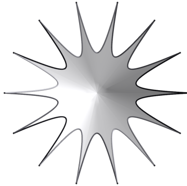
Klein quartic, genus 3: 14-gon, Klein's pairing
