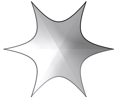
N_3 , nonorientable, \chi = -1 : hexagon, word aabbcc
