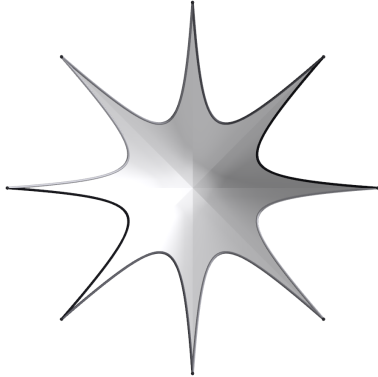
Bolza surface, genus 2: octagon, opposite sides paired
