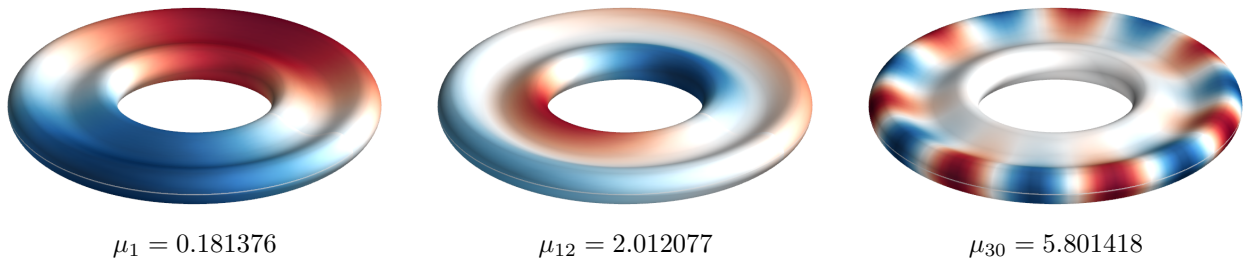
Figure 10: Eigenfunctions of the discocyte torus at three points of the spectrum, d = 6 , r = 1 on a 12 \times 12 mesh of the flat torus, drawn on the surface with a common color scale; the fields close up across both identifications. Sign arbitrary.
