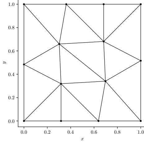
Figure 1: Sixteen-triangle unstructured mesh used in all numerical experiments.
