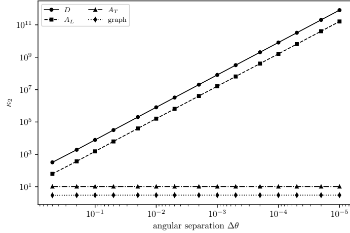
Figure 3: Condition numbers as two redundant local directions coalesce. The mesh, discrete dimension and Helmholtz problem are fixed; only the angular separation changes.
