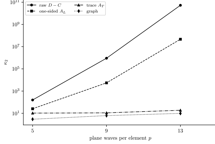
Figure 2: Condition numbers under local plane-wave enrichment. Raw and one-sided conditioning inherit the deterioration of the plane-wave coordinates, whereas the symmetric trace and graph representations remain moderate.
