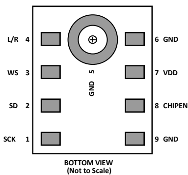
Figure 3. Pin Configuration
