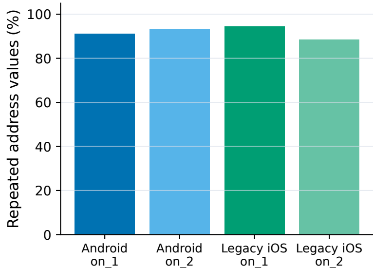
Observed private-address value repetition
