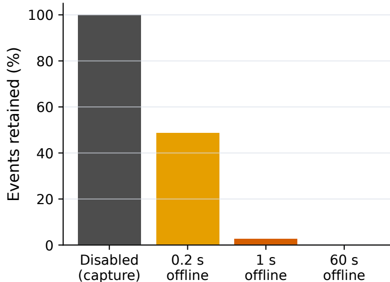
Duplicate-filter replay over captured events
