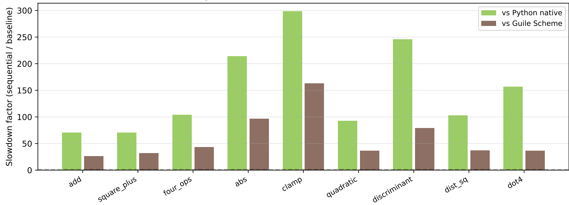
GNN Sequential Evaluator Overhead vs. Native Execution
