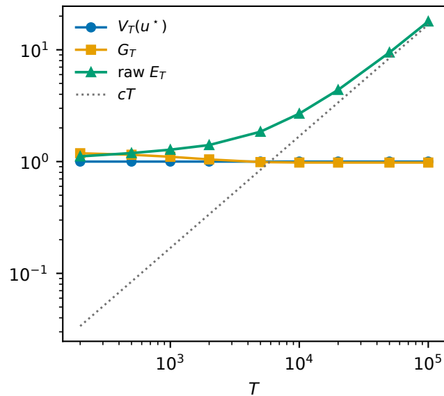
Raw separation: V_T, G_T = O(1) ; E_T \propto T
