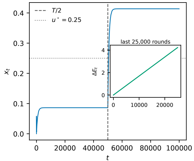
Two settled regimes, T = 10^5
