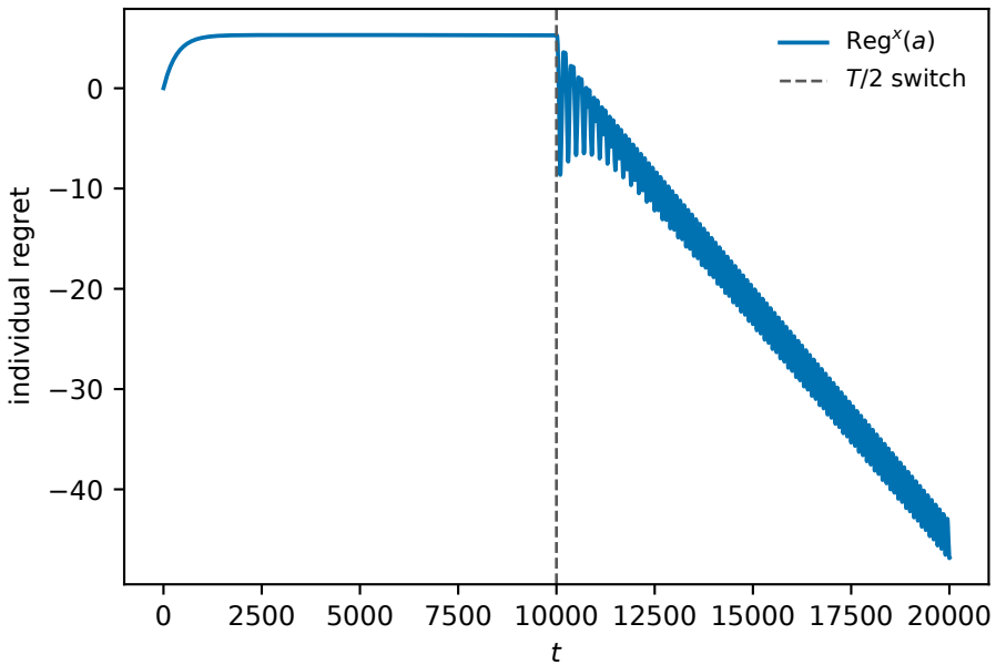
G2 same-run switch (continuous at b )
