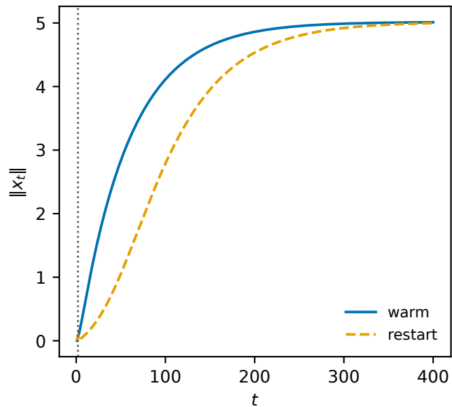
origin jump after one reset
