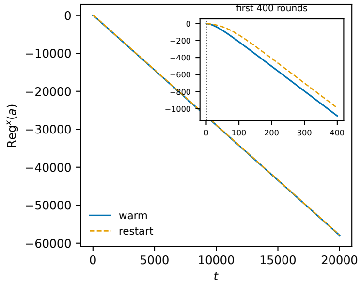
constant gap, parallel tails
