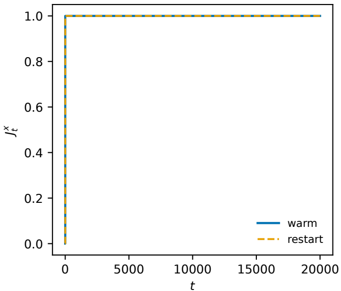
vs y \equiv e_1 : finite doubling
