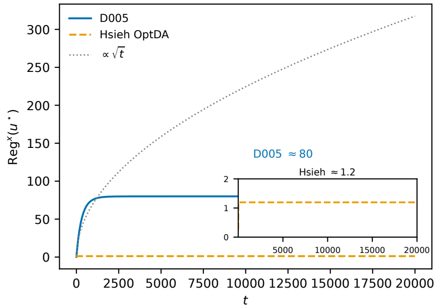
G3 constant opponent, V_T(u^*) = 0
