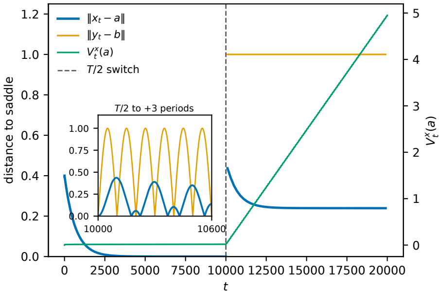
G2 same-run switch (no reset)
