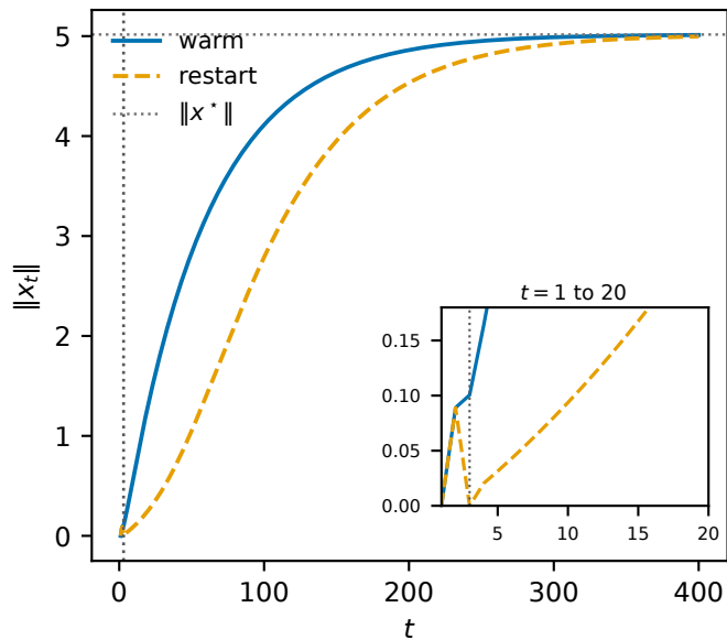
re-climb toward x^*
