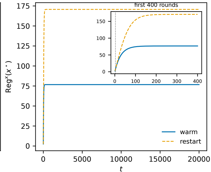
regret at x^* : constant offset
