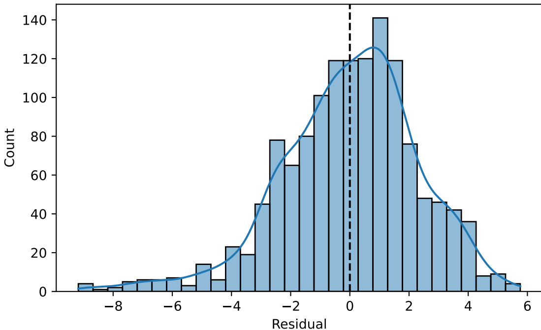
LOSO: Residual Distribution
