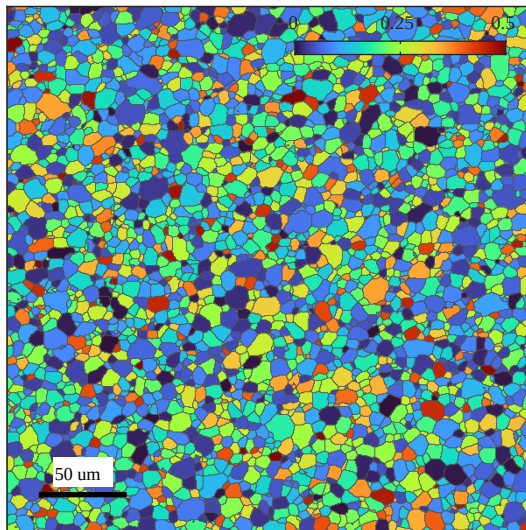
(a) 7d: Basal \langle a \rangle
