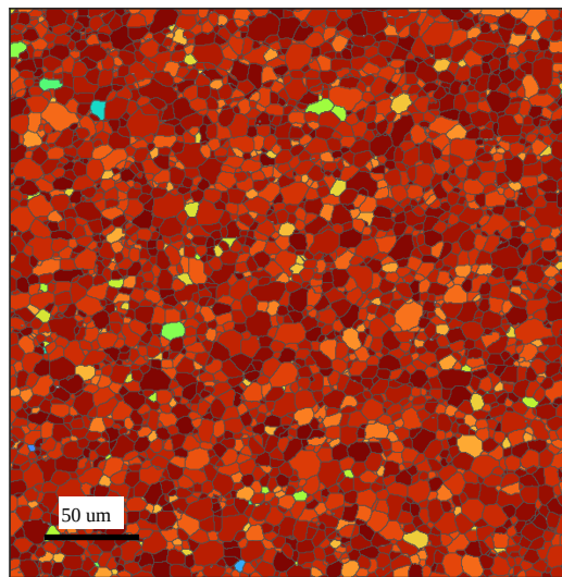
(b) 7d: Prismatic \langle a \rangle
