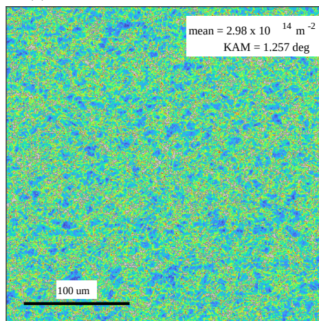
(b) 6.48d: 6.48 mm, 14.31% reduction
