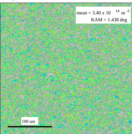
(g) 5.25d: 5.25 mm, 43.75% reduction
