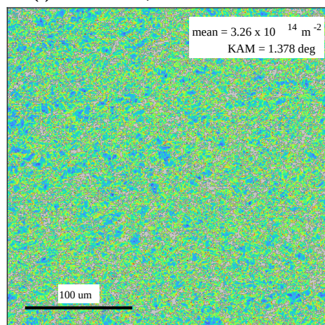
(e) 5.6d: 5.60 mm, 36.00% reduction
