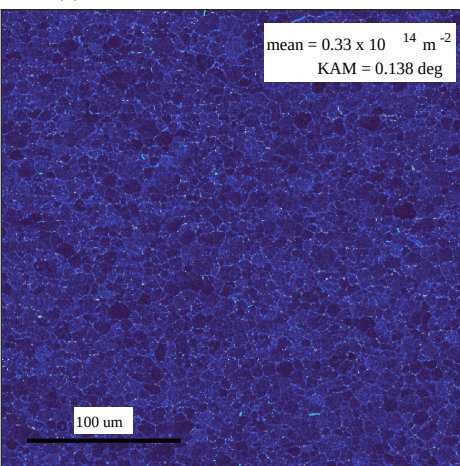
(a) 7d: 7.00 mm, 0.00% reduction
