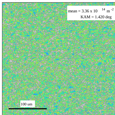
(h) 5d: 5.00 mm, 48.98% reduction
