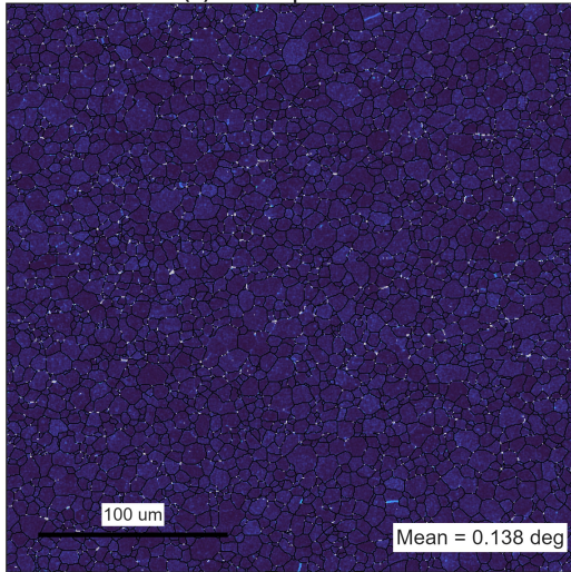
(a) 0.00% | 7.00 mm
