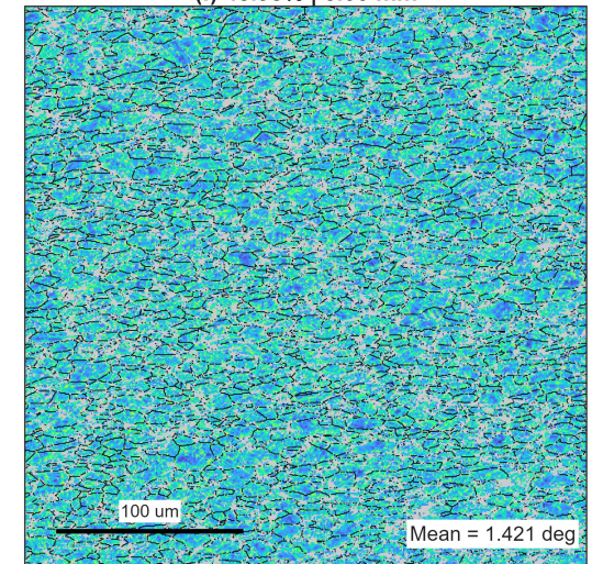
(f) 48.98% | 5.00 mm
