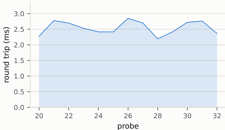
Application round trip through the relay
