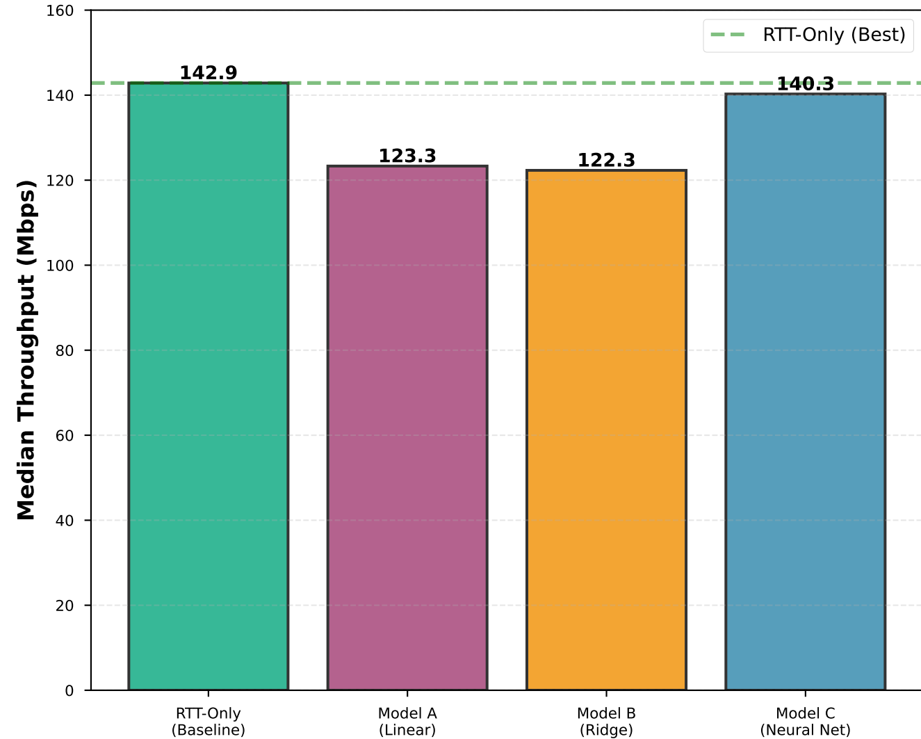
Server Selection Performance
