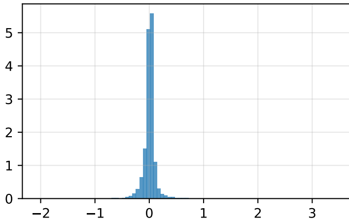
Random forest
