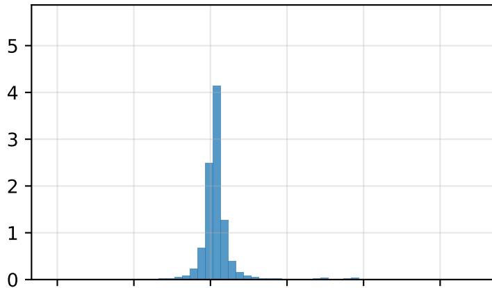
Random forest
