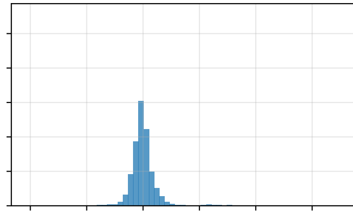
Ridge regression
