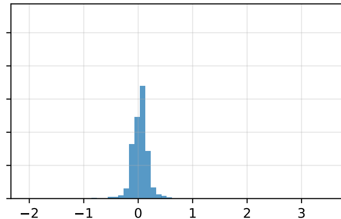
LSTM
