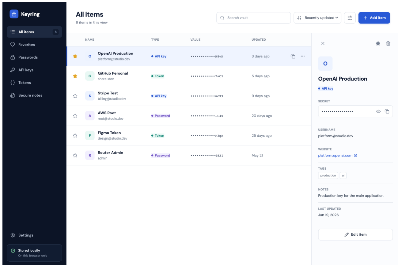
Figure 2. Selecting a row opens the detail inspector.
