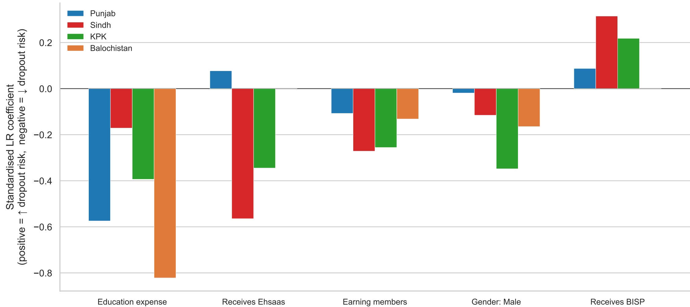
Top 5 Actionable Dropout Predictors by Province (Logistic Regression, balanced weights, standardised features, test-set AUC)
