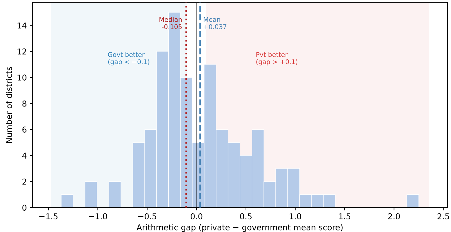
Histogram of District-Level Arithmetic Gaps (n = 102 filtered districts)
