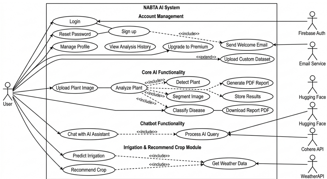
Figure 4.2. NABTA Use Case Diagram
