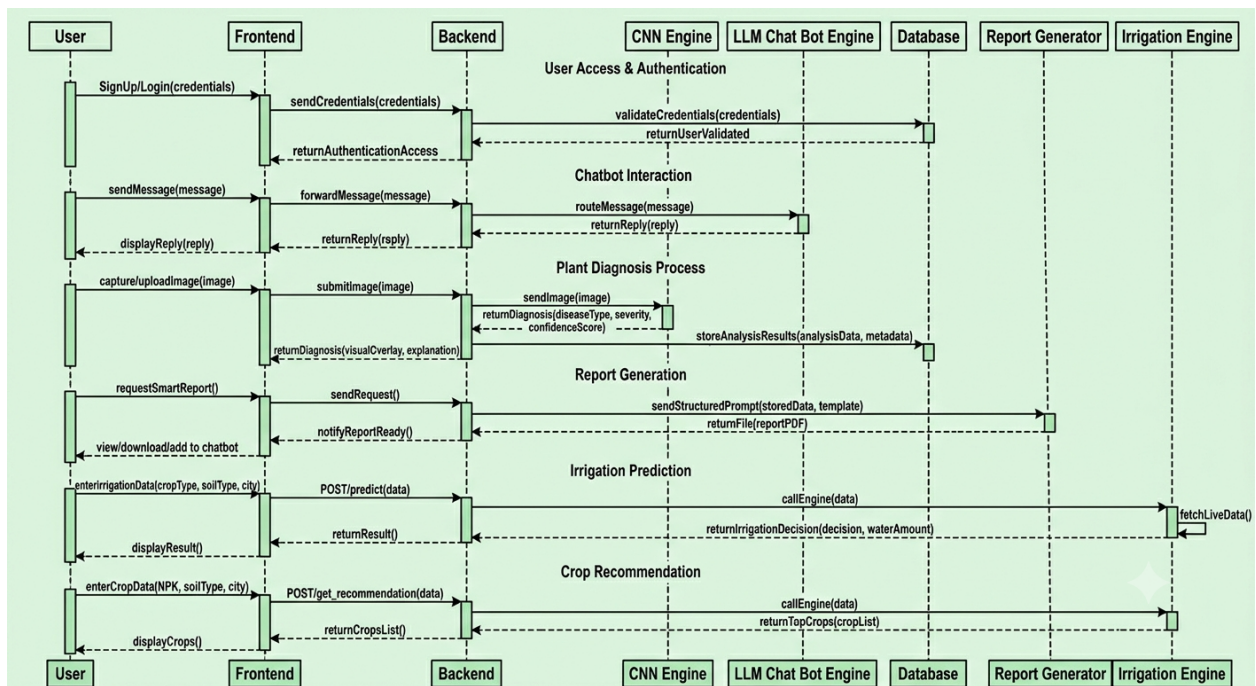
Figure 4.4. NABTA Sequence Diagram
