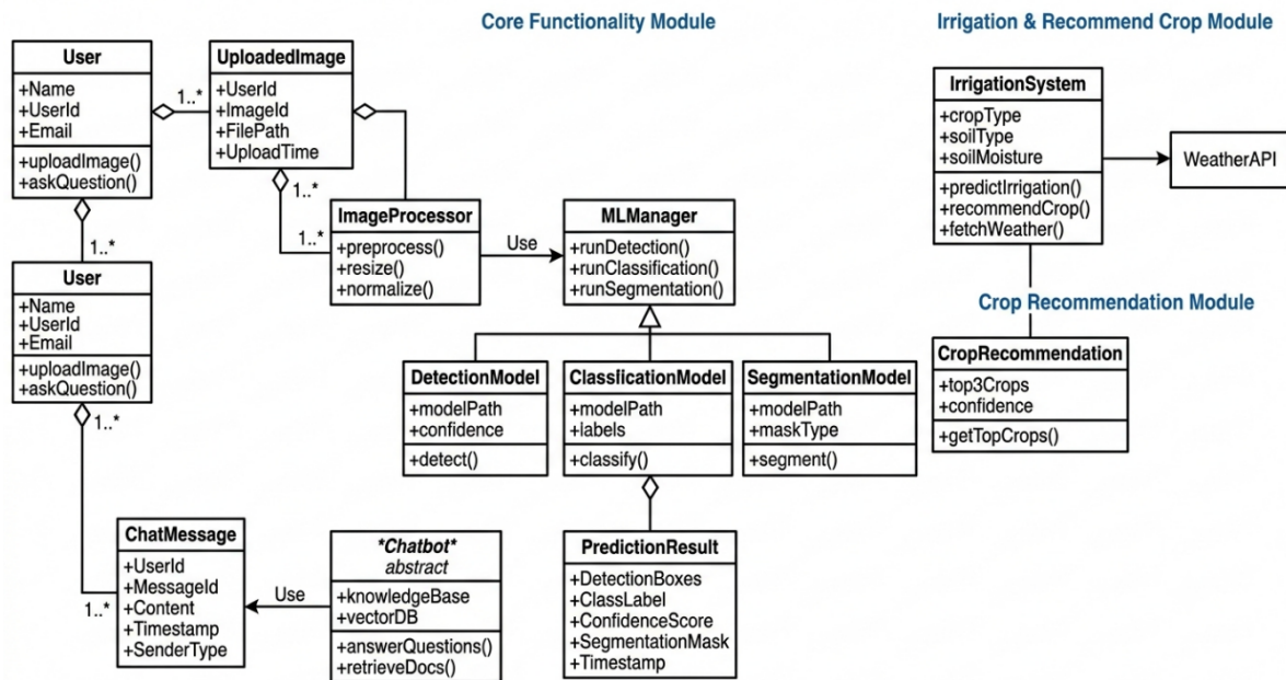
Figure 4.5. NABTA Class Diagram
