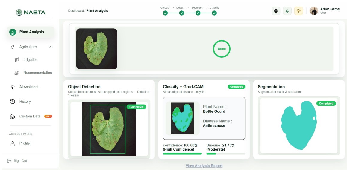
Figure 5.2. Analysis Results Screen with Detection, Segmentation, and Grad-CAM Panels
