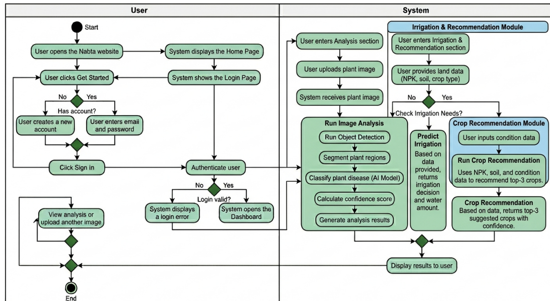
Figure 4.3. NABTA Activity Diagram
