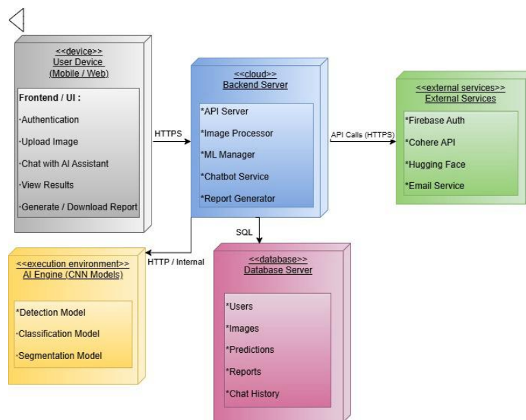
Figure 4.8. NABTA Deployment Diagram
