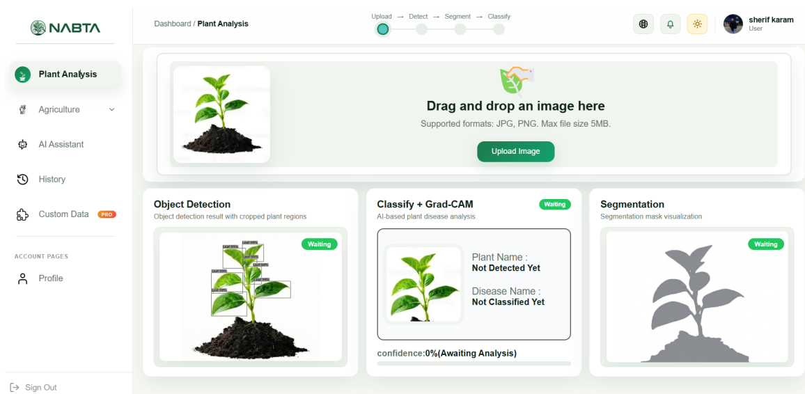
Figure 4.9. NABTA Main Analysis Dashboard Interface
