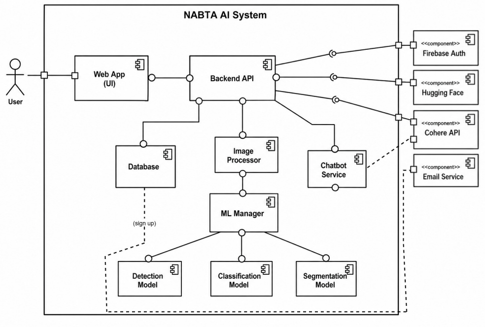
Figure 4.7. NABTA Component Diagram
