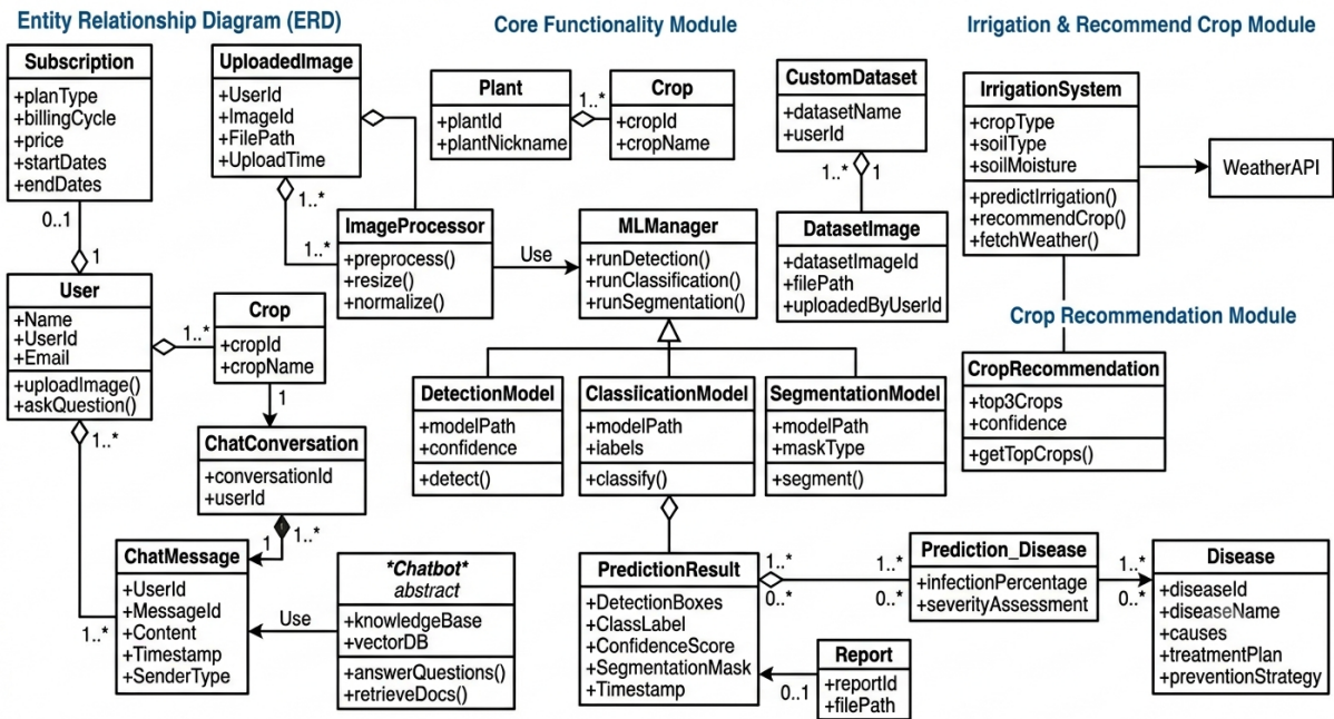
Figure 4.6. NABTA Entity Relationship Diagram
