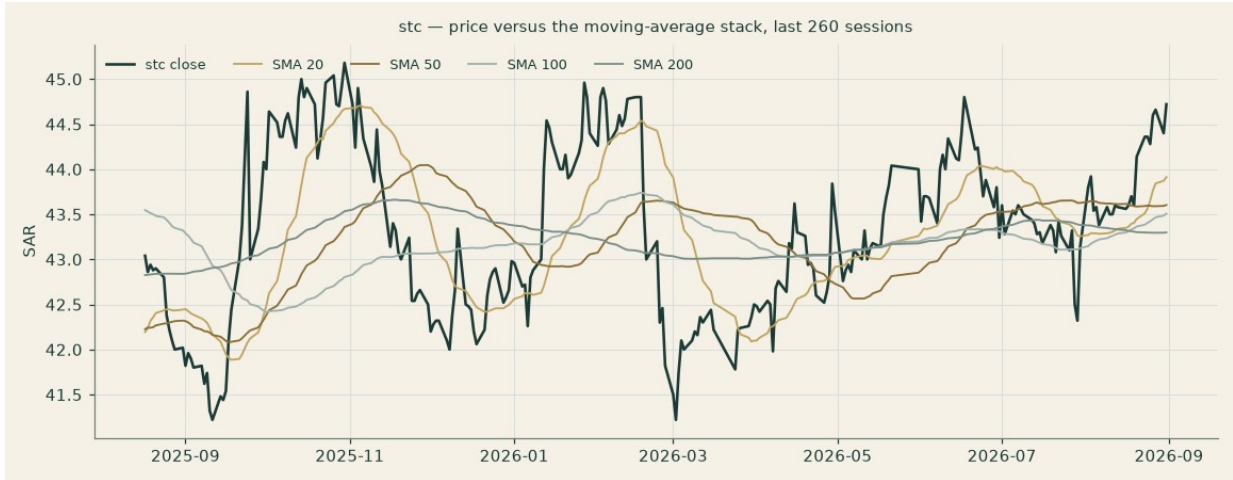
Figure 3 — Price against the moving-average stack, the last 260 sessions.
