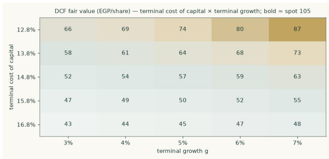
Figure 3 — discounted-cash-flow fair value per share across the terminal cost of capital and terminal growth. Bold cells sit within EGP 6 of the market price of 105.20.
