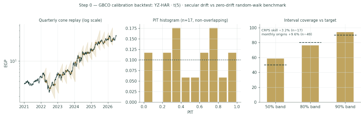
Figure B-1 — Calibration backtest: quarterly cone replay (log scale), PIT histogram, and interval coverage versus target, secular-drift configuration.
