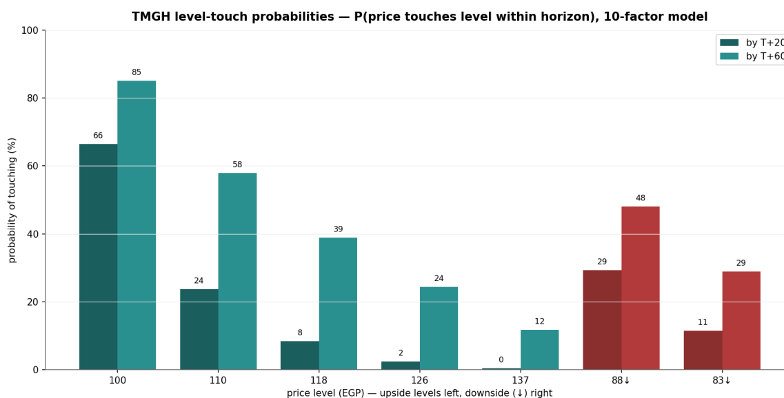
Figure 5. Level-touch probabilities (10-factor model) — probability of the price touching each level within each horizon (T+20 / T+60): upside 100 = 66%/85%, 110 = 24%/58%, 118 = 8%/39%, 126 = 2%/24%, 137 = 0%/12%; downside 88 = 29%/48%, 83 = 11%/29%. A descriptive output of the simulation: how often paths reach each level, nothing more.
