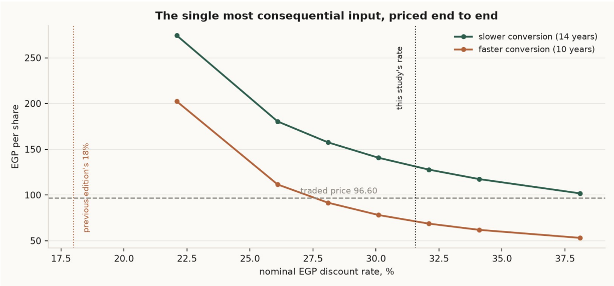
The discount rate against value per share, on both readings of the order book. The dotted lines mark this study's rate and the 18% the June 2026 edition used.
