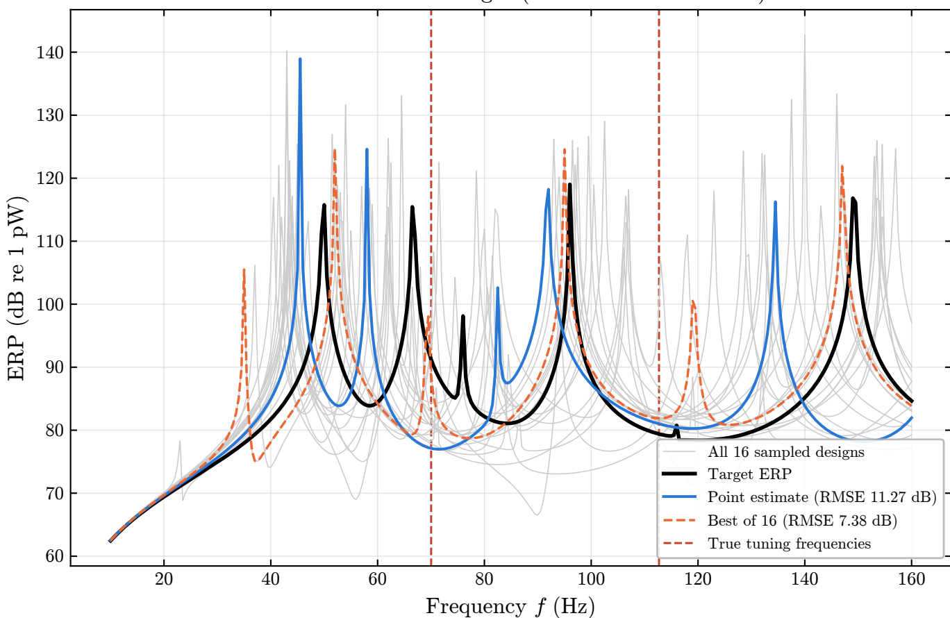
iGNO: ERP of the designs (checked with the solver)
