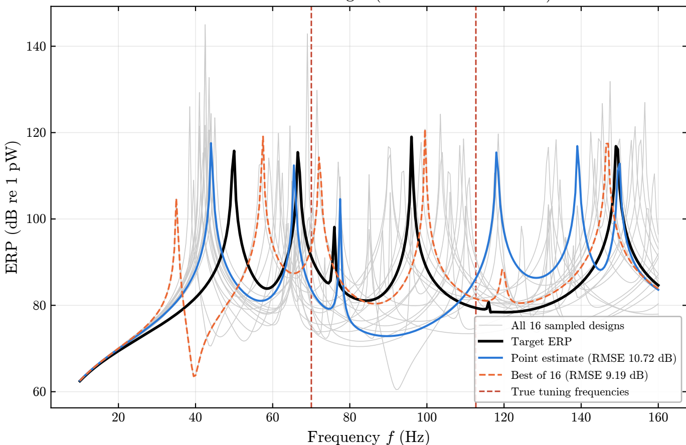
iSTO: ERP of the designs (checked with the solver)
