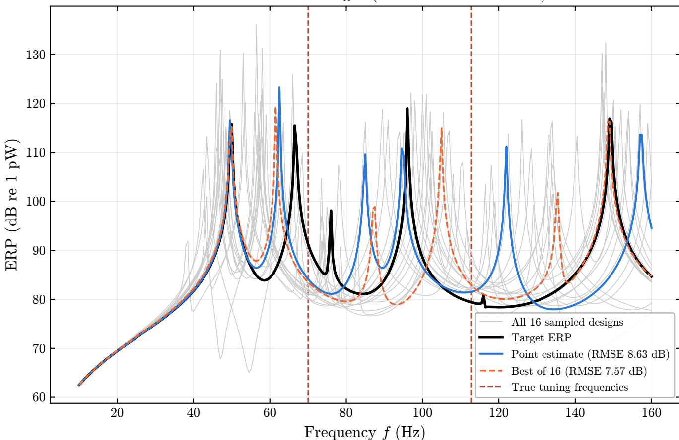
iLNO: ERP of the designs (checked with the solver)
