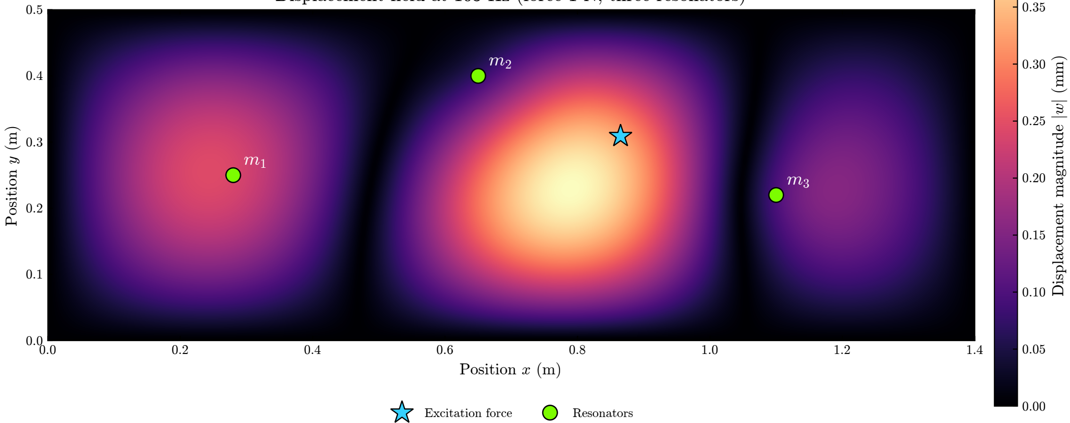
Displacement field at 103 Hz (force 1 N, three resonators)
