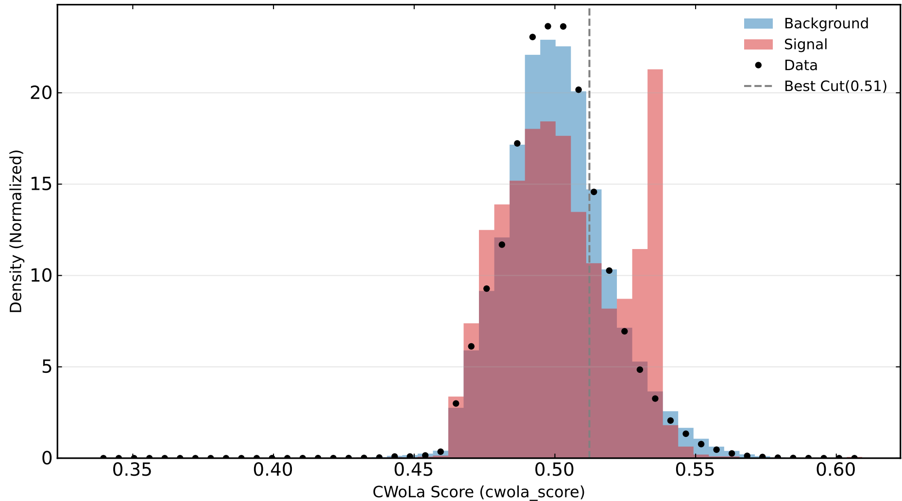
CWoLa Classifier Score Distributions
