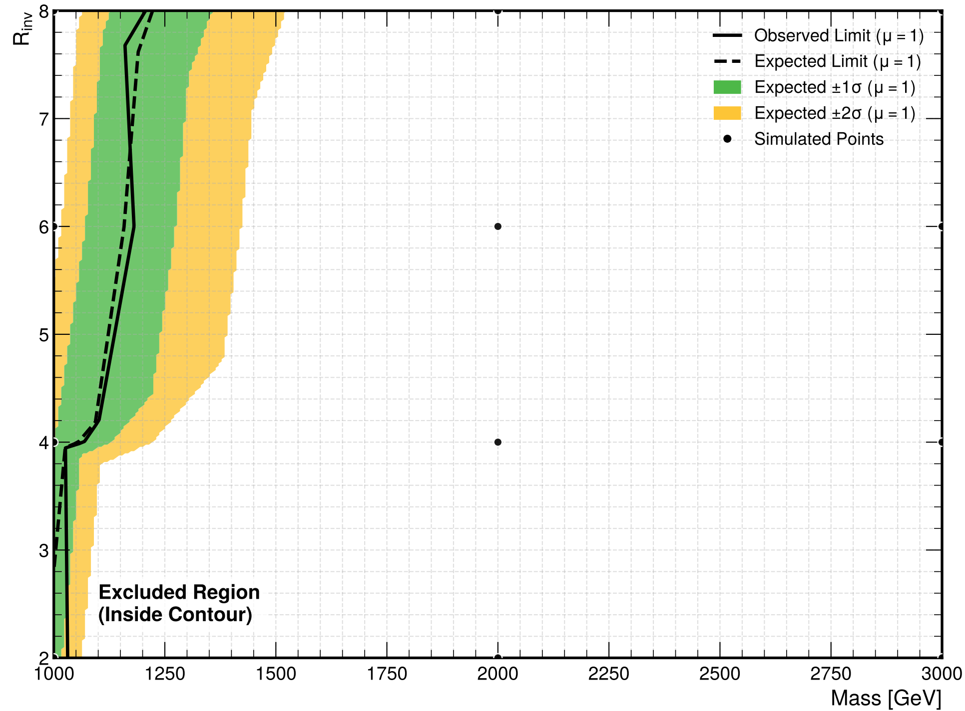
2D Brazilian Exclusion Contour (PyHF)
