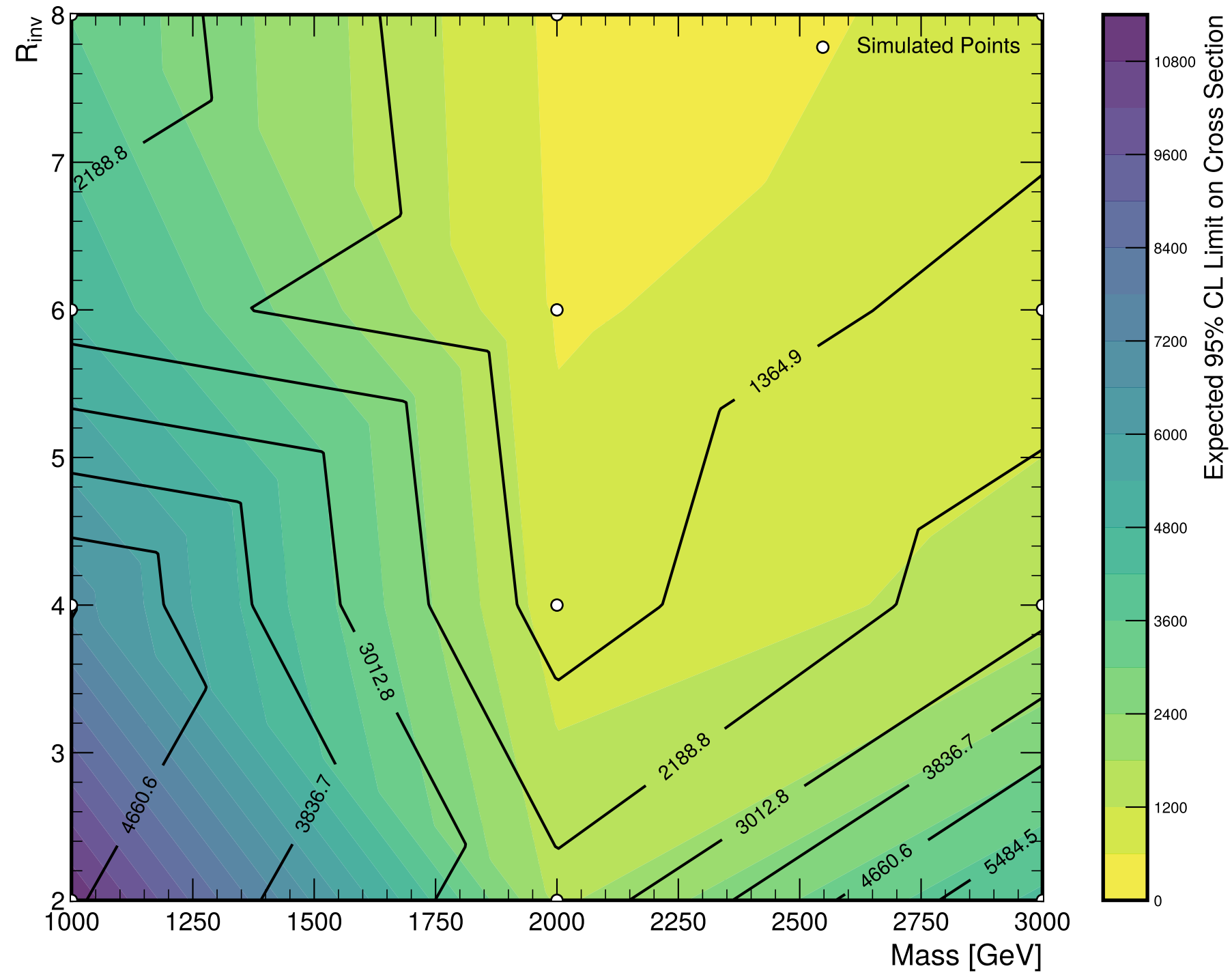
2D Limit Heatmap (Cross Section)
