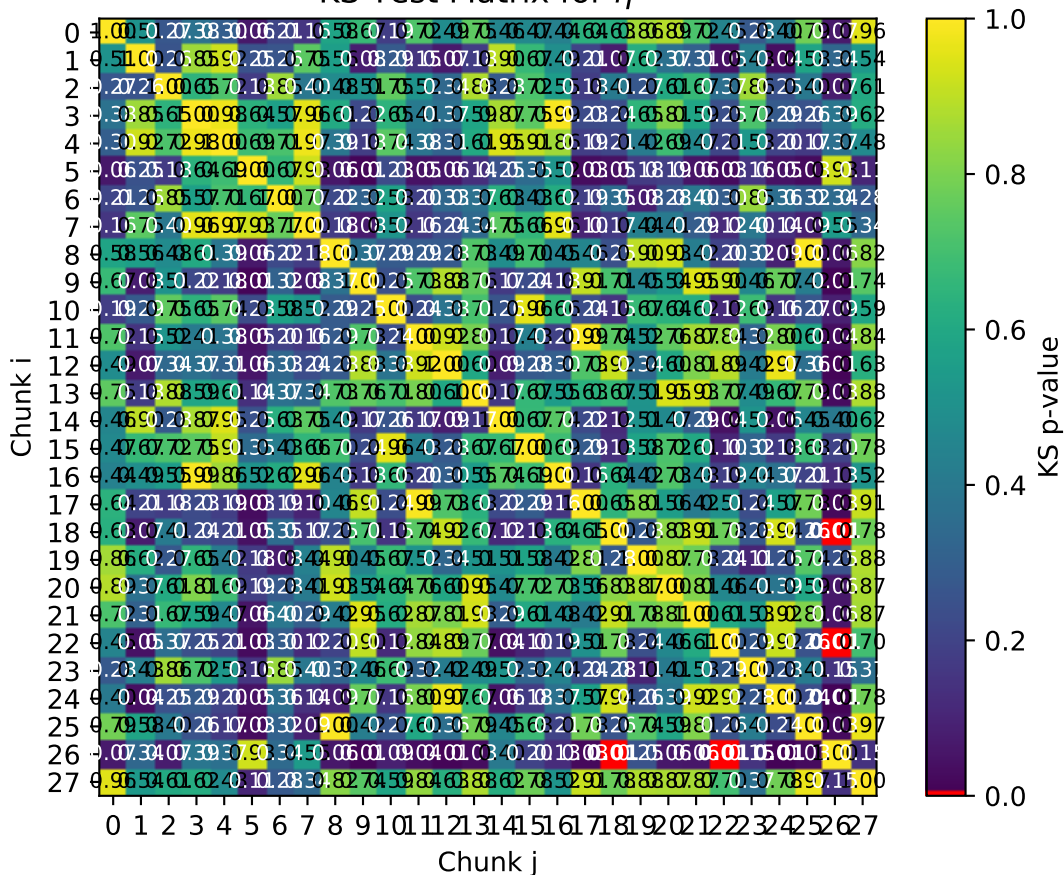
KS Test Matrix for \eta^{j1}
